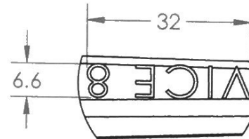
DETAIL B SCALE 1 : 1
