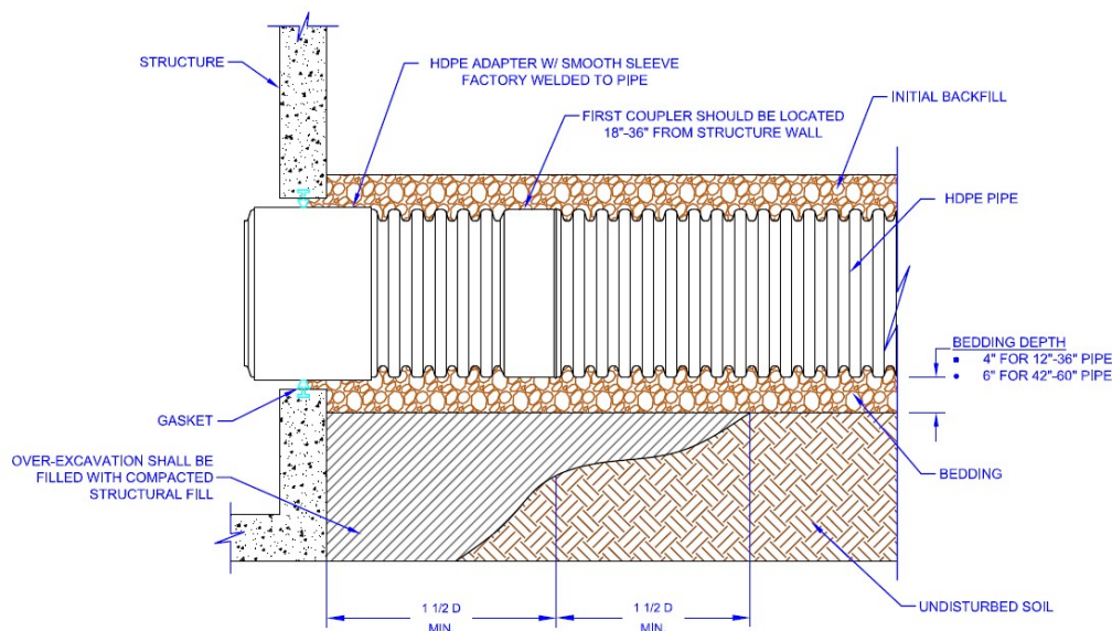
Figure 6 - Typical Structure Connection
