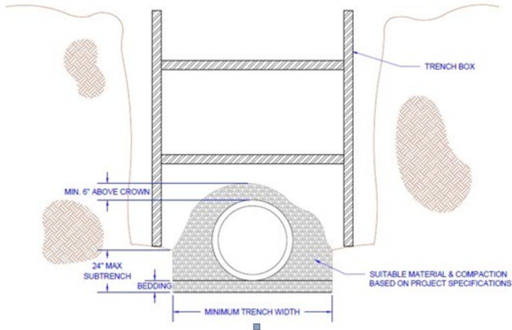
Figure 4 - Typical Sub-Trench Installation
