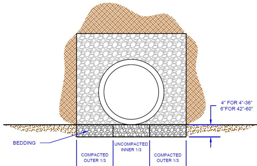
Figure 7 - Bedding Placement
