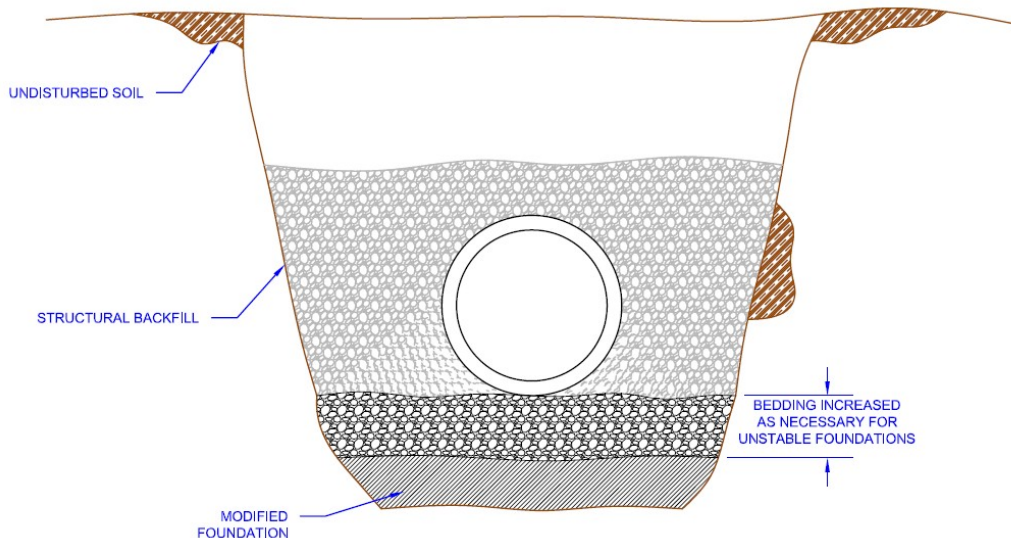
Figure 5 - Modified Foundation
